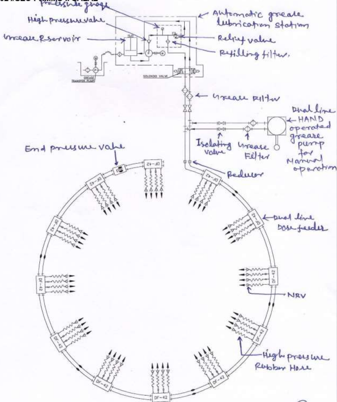
CHART OF LUBRICATION POINTS
