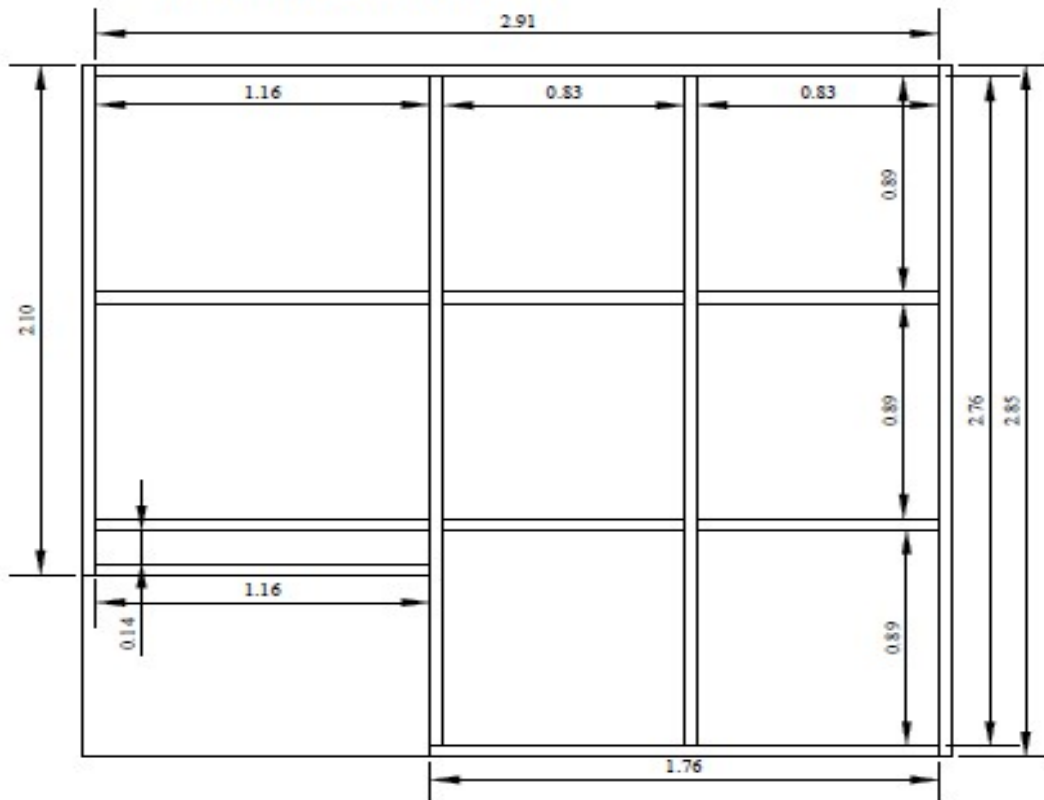
LIFT ROOM PART-I
