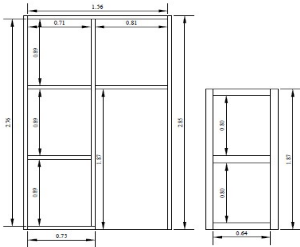
LIFT ROOM PART-II LIFT ROOM DOOR
