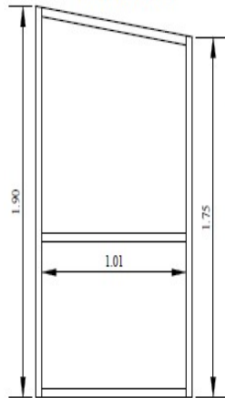
OPEN SPACE RIGHT PART-IV ABOVE LANDING
