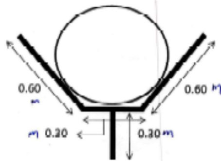
MS ANGLE FENCING WITH CONCERTINA COIL
