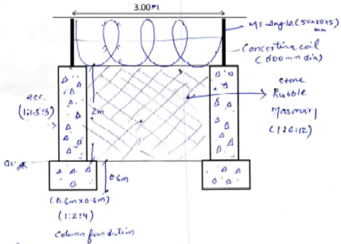
MS ANGLE FENCING WITH CONCERTINA COIL
