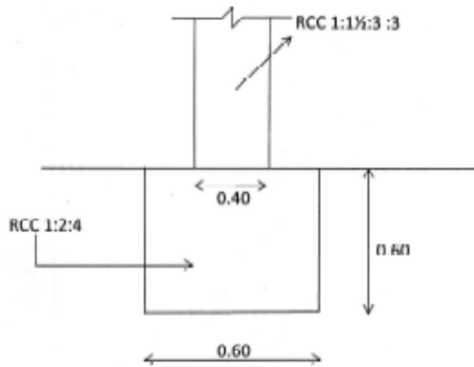
Column Cross-Section
