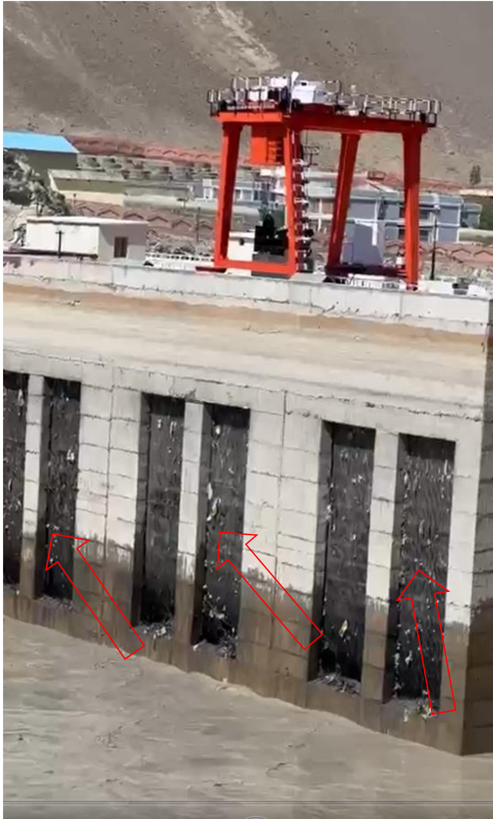
Trash Rack filled with branches , plastic bottles, sacs, polythene and other unwanted materials
