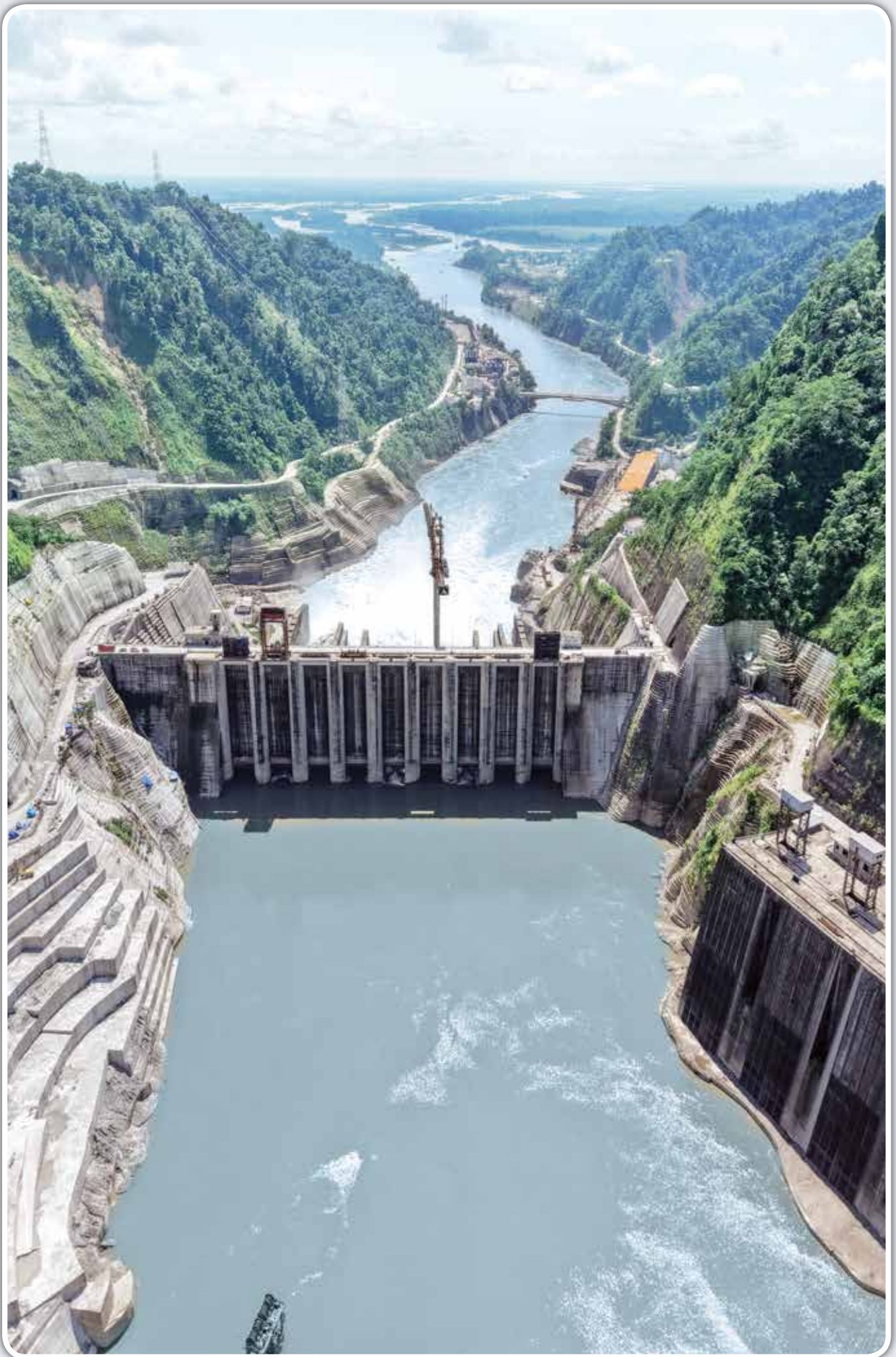
2000 MW Subansiri Lower HEP (Assam / Arunachal Pradesh) - Dam
